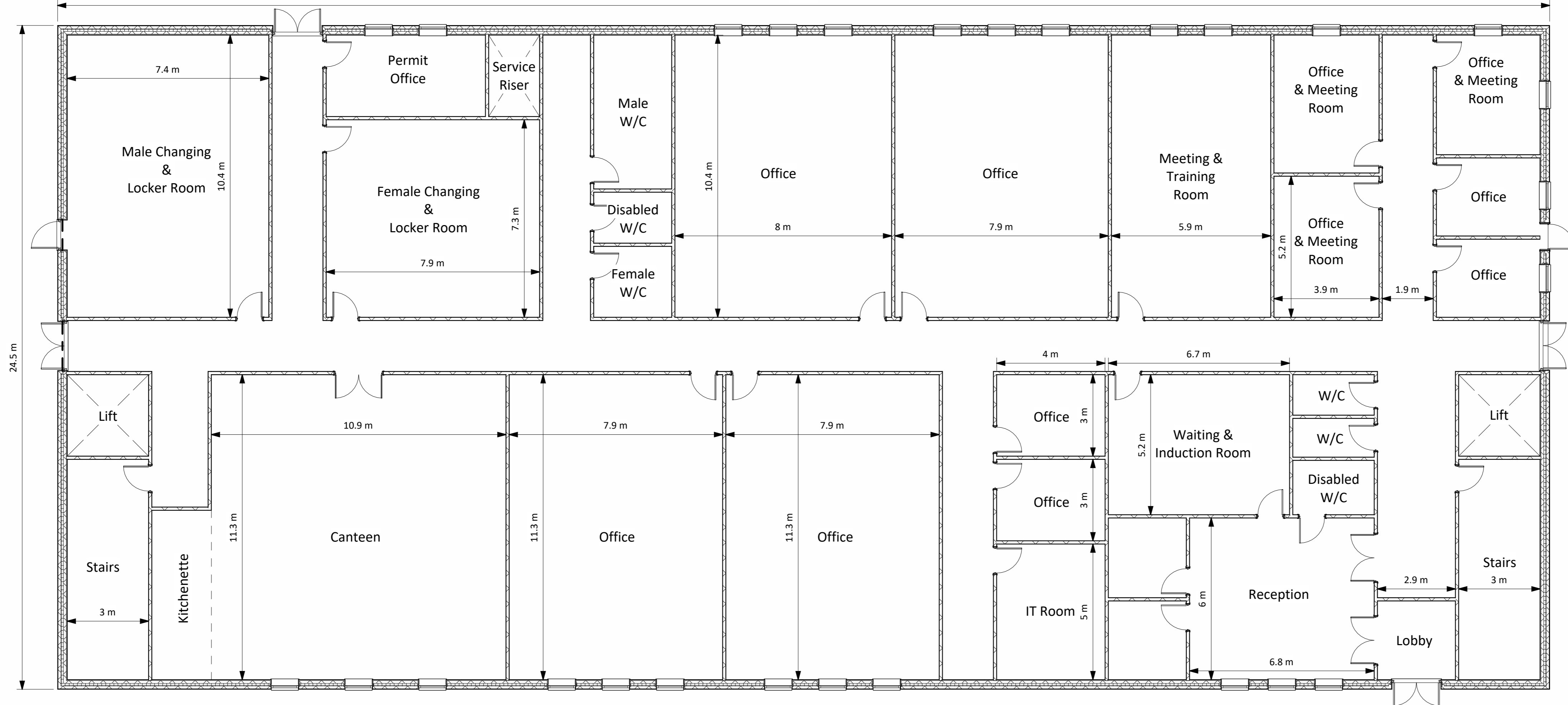
1 Admin Building Ground Floor 85.250m AOD 1 : 100
