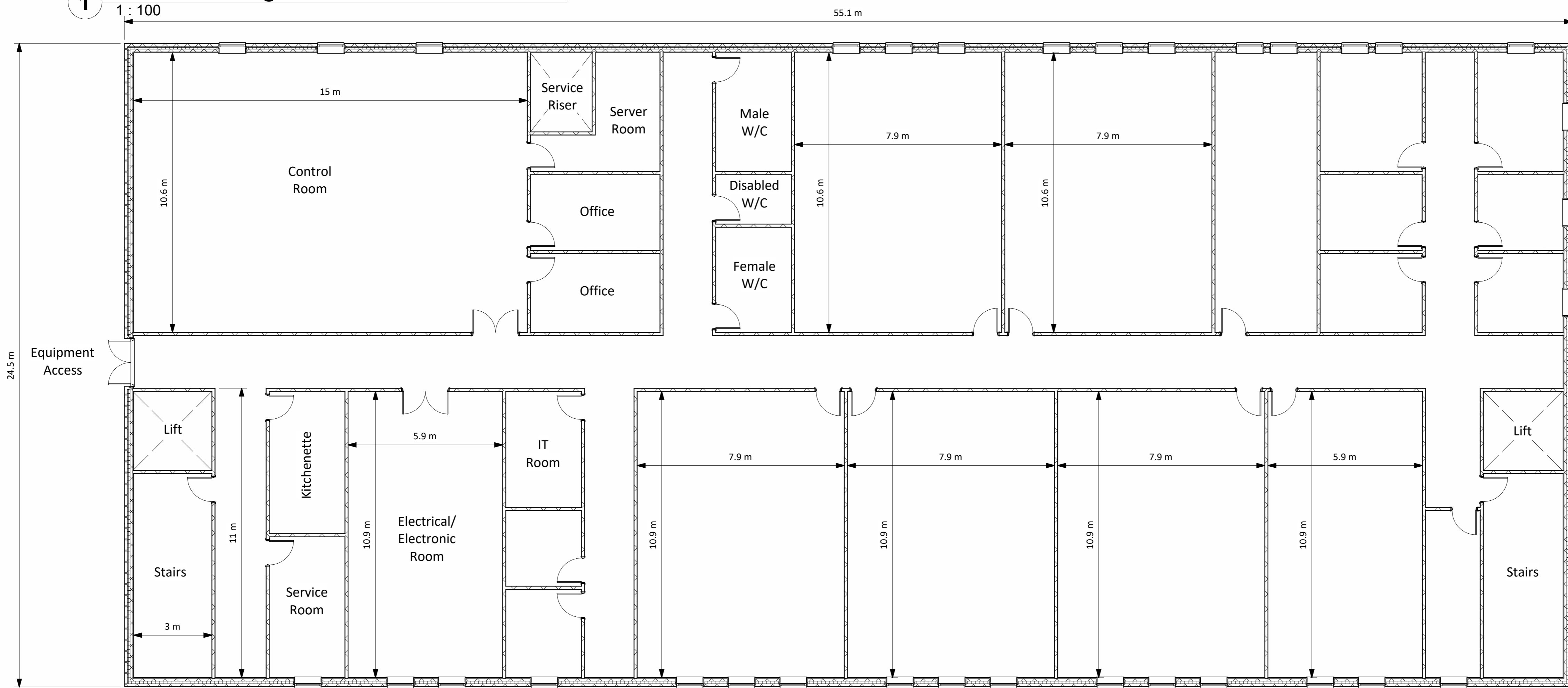
2 Admin Building First Floor 89.250m AOD 1 : 100
